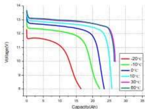
Discharge Curves at Different Temperature
